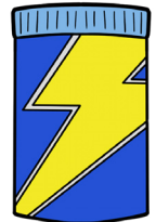
ELECTROLYTES
